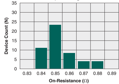
Typical On-Resistance Distribution (N=50, I F =5mA, I L =600mA)
