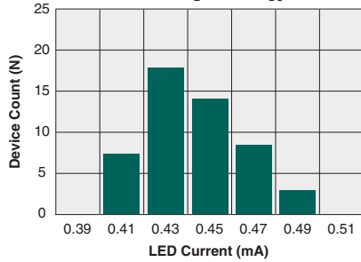
Typical I F for Switch Operation (N=50, I L =600mA DC )
