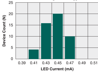
Typical I F for Switch Dropout (N=50, I L =600mA DC )
