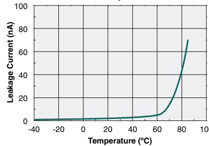
Typical Leakage Current vs. Temperature
