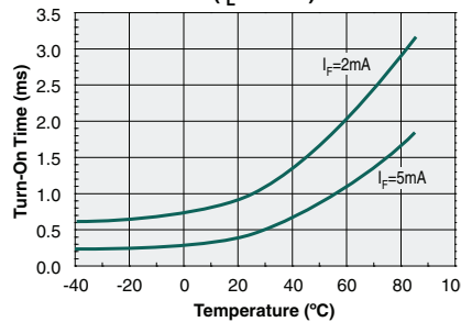
Turn-On Time vs. Temperature (I L =55mA)
