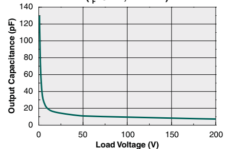
Output Capacitance vs. Load Voltage ( I_F=5mA, f=1MHz )
