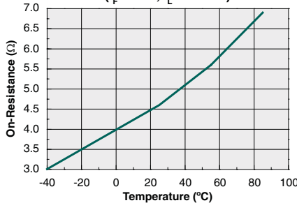
On-Resistance vs. Temperature DC-Only Configuration ( I_F=0mA, I_L=100mA )
