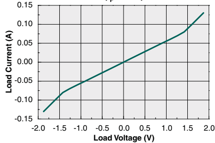
Typical Load Current vs. Load Voltage AC/DC Configuration ( I_F=0mA )
