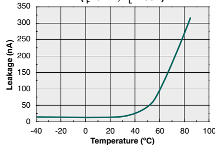
Typical Leakage vs. Temperature Measured Across Pins 4&6 ( I_F=5mA, V_L=400V )
