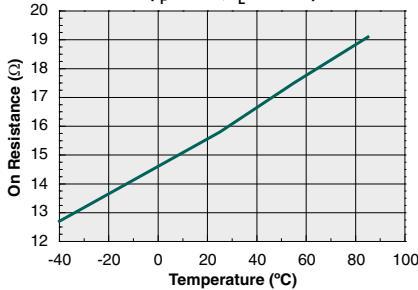
On-Resistance vs. Temperature AC/DC Configuration ( I_F=0mA, I_L=75mA )
