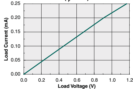
Typical Load Current vs. Load Voltage DC-Only Configuration ( I_F=0mA )
