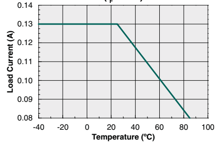
Maximum Load Current vs. Temperature - AC/DC Configuration ( I_F=0mA )
