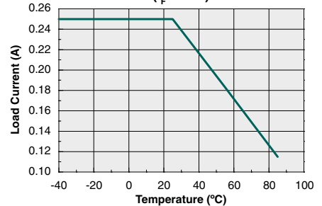
Maximum Load Current vs. Temperature - DC Configuration ( I_F=0mA )
