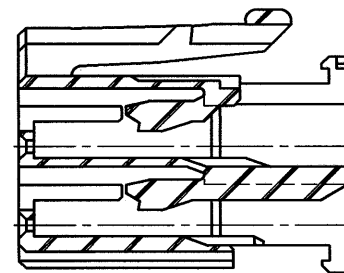
SECT. B-B
