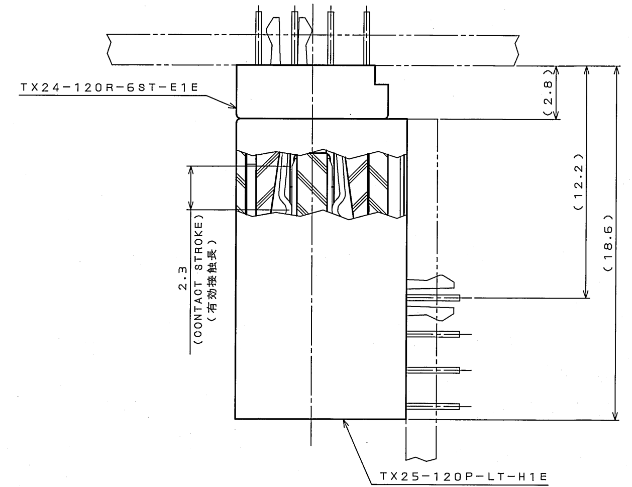
MATED CONDITION (REF.) 嵌合状態図 (参考) (SCALE 5:1)
