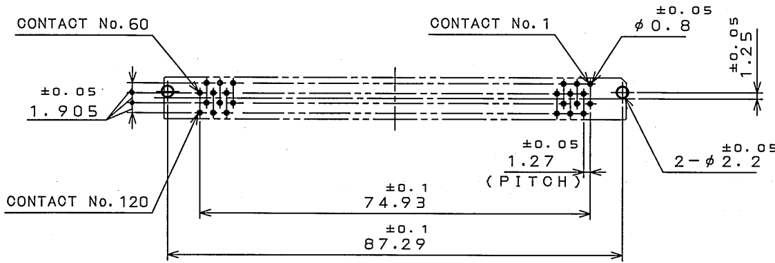
APPLICABLE P.C.B. DIMENSION (REF.) 適合基板寸法 (参考) (SCALE 1:1)
