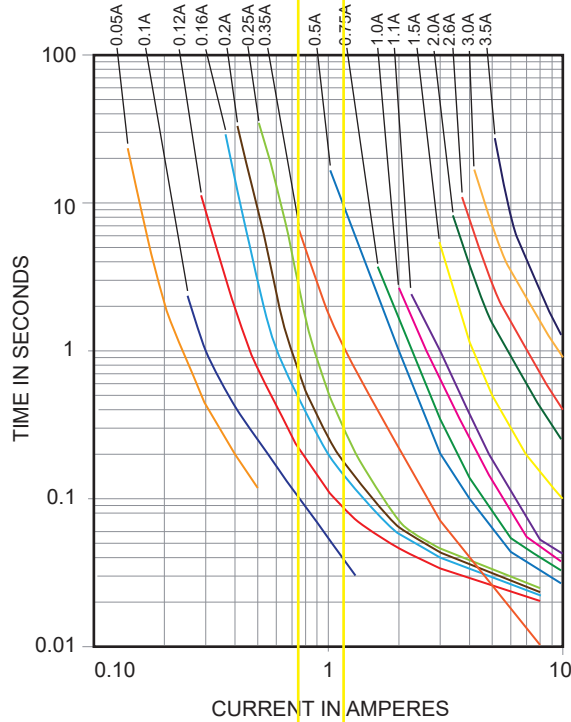
Thermal Derating Chart
