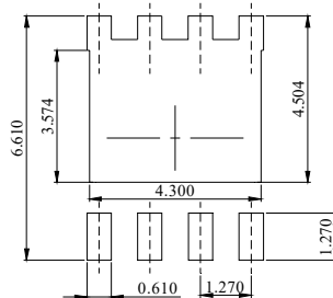
DIMENSIONS: MILLIMETERS
