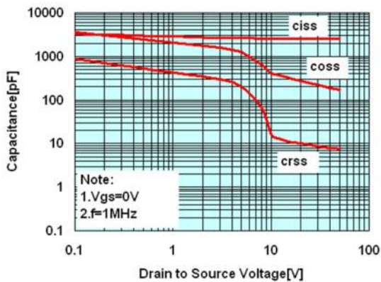
Capacitance Characteristics
