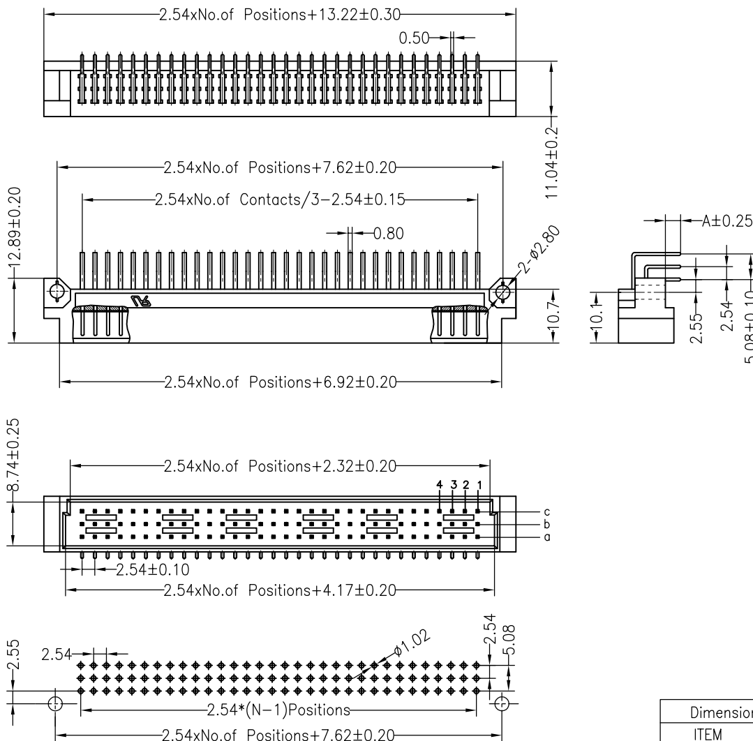
Recommended P.C.B Layout(Top Side) (PCB BOARD TOLERANCE±0.05)
