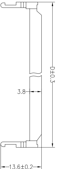
Strain relief P/N: G5315-XXDB01
