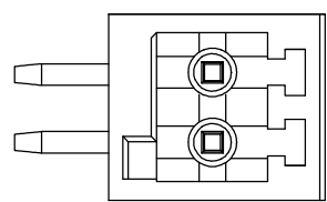
Recommended P.C.B Layout(Top Side) 02P
