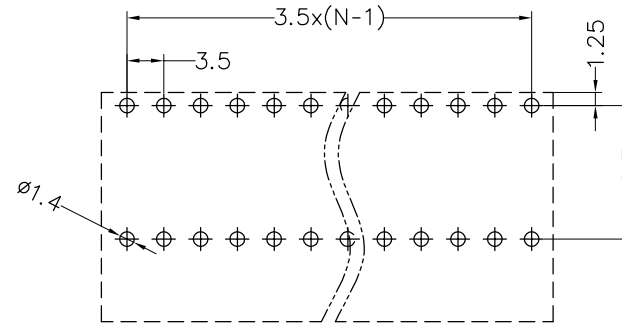
PCB LAYOUT
