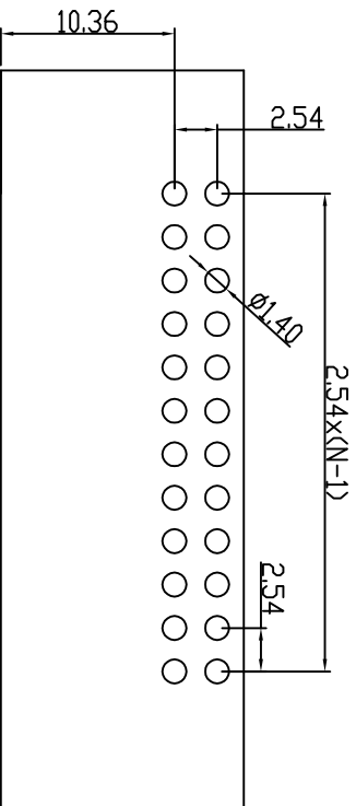
PCB LAYOUT
