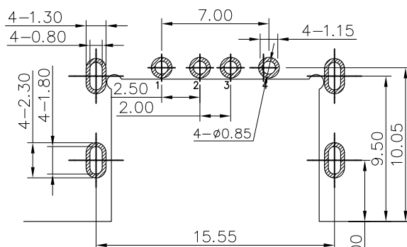
RECOMMENDED P.C.B HOLE LAYOUT COMPONENT SIDE VIEW(TOLERANCE: +/-0.05)
