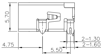
RECOMMENDED P.C.B HOLE LAYOUT COMPONENT SIDE VIEW(TOLERANCE: +/-0.05)
