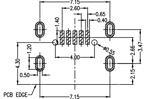
RECOMMENDED PCB LAYOUT PCB图仅供参考
