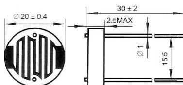
Dimensions in millimetres
