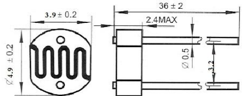
Dimensions in millimetres
