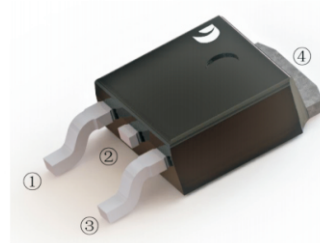
TO-252(D-PAK)
