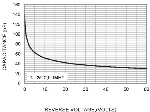
FIG.3-TYPICAL JUNCTION CAPACITANCE
