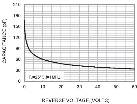
FIG.3-TYPICAL JUNCTION CAPACITANCE
