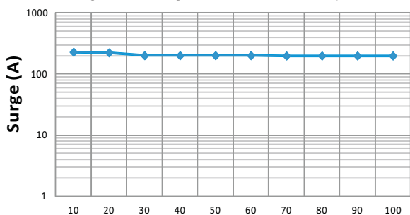
Fig.3 Derating Curve for number of pulses
