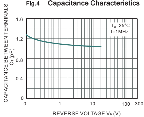
Fig.4 Capacitance Characteristics
