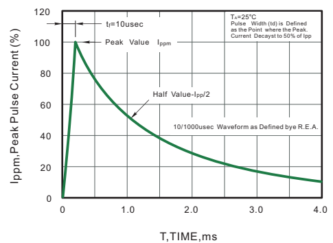
Fig.8 Pulse Waveform
