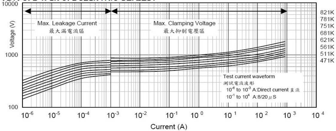
VDR-07D471k-07D821k (N/J SERIES)
