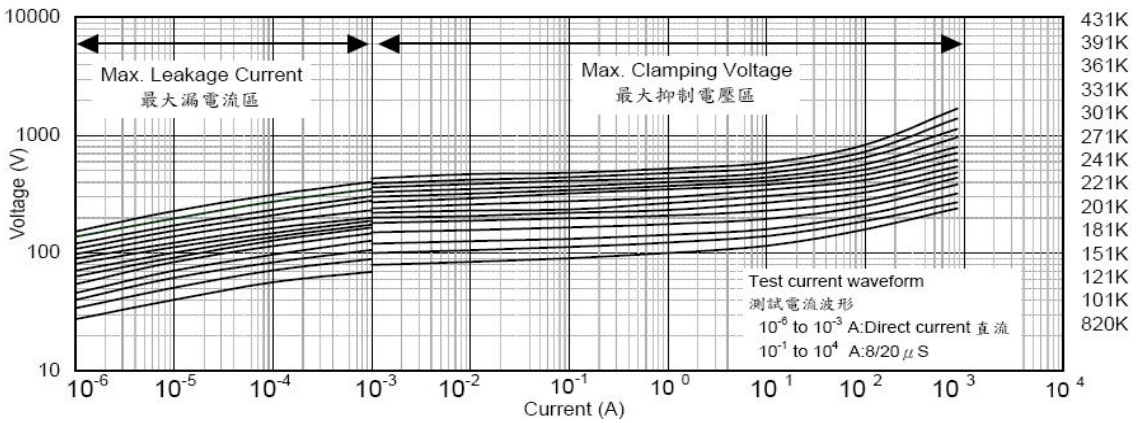
VDR-07D820k-07D431k (N/J SERIES)
