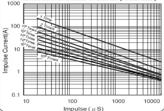
VDR-07D080M-07D180L-07D681k (N SERIES)
