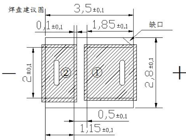
焊盘建议大小 Recommended size of pad
