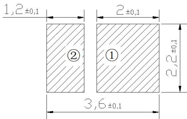
焊点结构 Pad Configuration:
