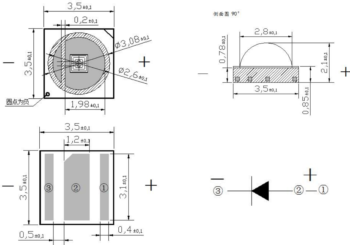
焊盘建议大小 Recommended size of pad
