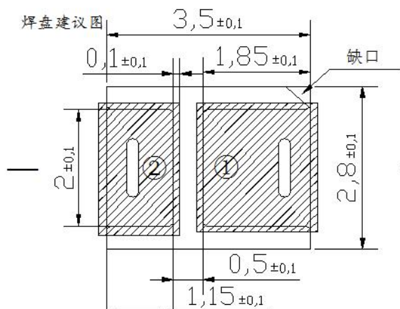
焊盘建议大小 Recommended size of pad
