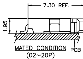
MATED CONDITION (02~20P)
