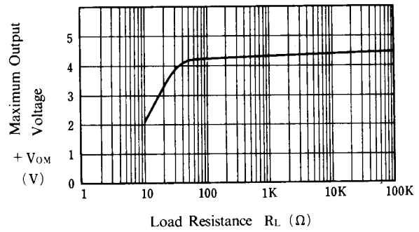
Maximum Output Voltage vs. Load Resistance ( V^+ = 5\text{V} , T_a = 25^\circ\text{C} )
