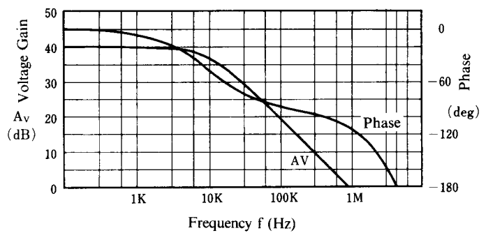
Voltage Gain, Phase vs. Frequency ( V^+/V^- = \pm 4.3\text{V} , R_L = 2\text{ k}\Omega , A_V = 40\text{dB} , T_a = 25^\circ\text{C} )
