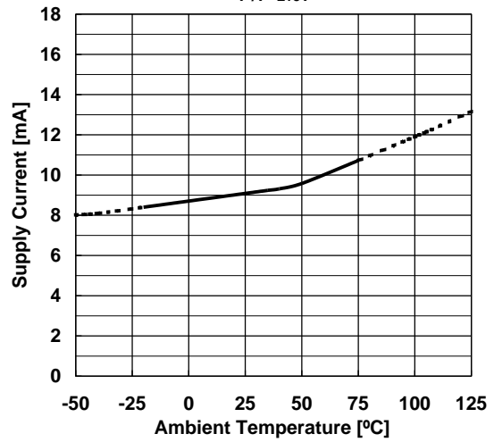
Supply Current vs. Temperature V+/V- = ±15V
