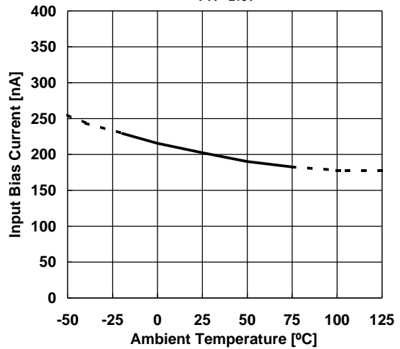
Input Bias Current vs. Temperature V+/V- = ±15V
