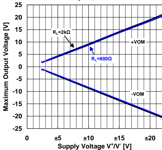
Maximum Output Voltage vs. Supply Voltage R L =2kΩ, Ta=25°C
