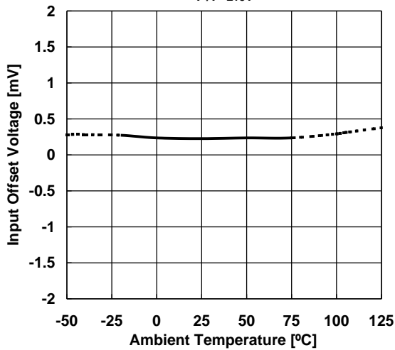
Input Offset Voltage vs. Temperature V+/V- = ±15V
