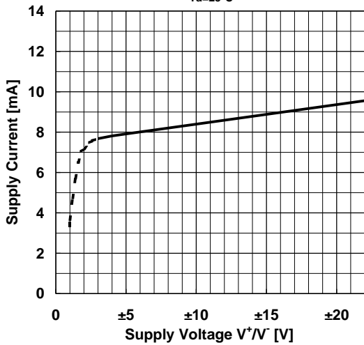
Supply Current vs. Supply Voltage Ta=25°C
