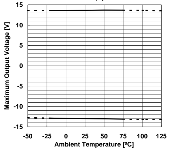
Maximum Output Voltage vs. Temperature V+/V- = ±15V, R L =600Ω
