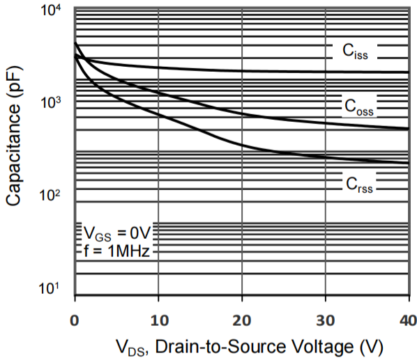
Figure 7. Capacitance
