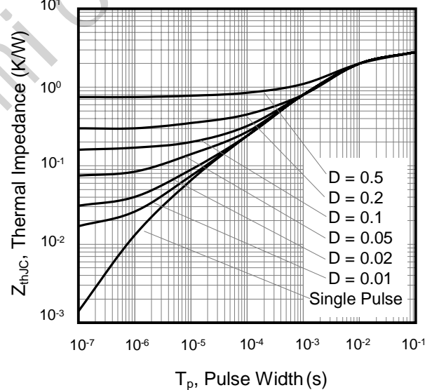
Figure 10. Transient Thermal Impedance TO-220, TO-3P
