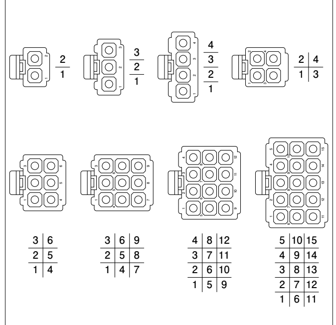
Plug housing
