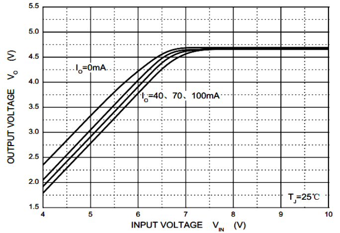
Dropout Characteristics
