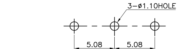
Recommended PCB Layout(Pattern Side) Top View tolerance: ±0.05mm
