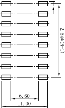
[P. C. B. LAYOUT]
