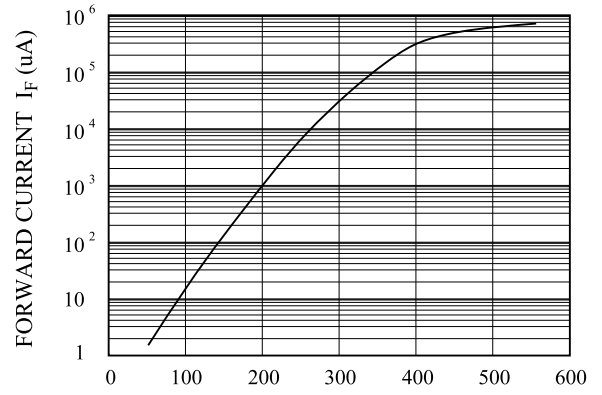
FORWARD VOLTAGE V_F (mV)
