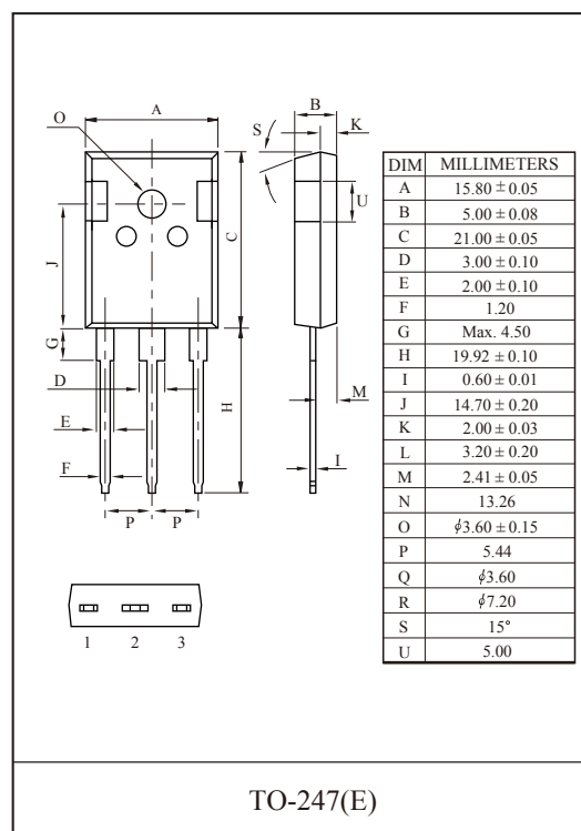
TO-247
