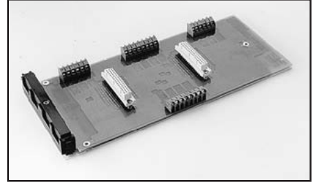
Model 7012-ST: Extra quick disconnect screw terminal board. One 7012-ST is included with each 7012-S. For use with: 7012-S
