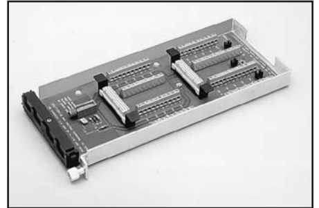
Model 7014-ST: Extra quick disconnect isothermal screw terminal board with cold junction sensor. One 7014-ST is included with each 7014. For use with: 7014
