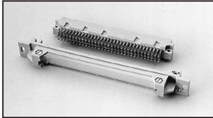
Model 7011-MTR: 96-pin male DIN connector with solder eyelets for bulkhead mount. Connects with the 7011-KIT-R and the 7011-MTC-2. For use with: 7011-KIT-R, 7011-C, 7012-C, 7013-C, 7015-C, 7018-C
