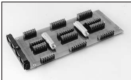
Model 7011-ST: Extra quick disconnect screw terminal board. One 7011-ST is included with each 7011-S. For use with: 7011-S
