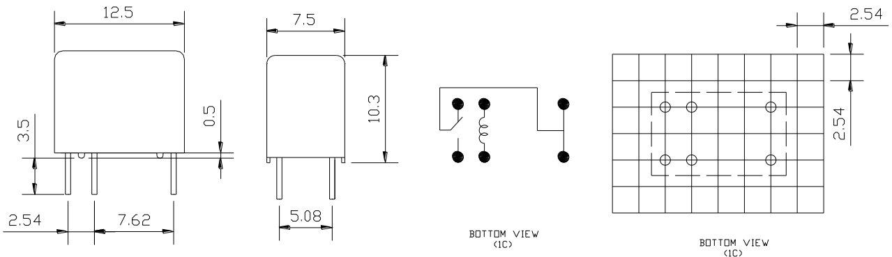
BOTTOM VIEW (1C)
