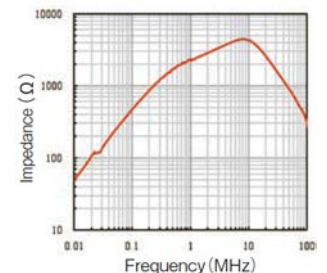
AF01-40 Impedance vs Frequency (10 turns)
