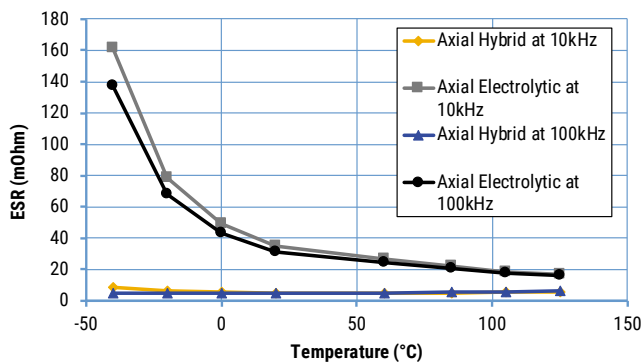
Temperature dependencies of ESR measured at 10 kHz and 100 kHz for Axial Hybrid (PHA225MKP3370QE4) and Axial Electrolytic (PEG226MG3370QE1) capacitors.
