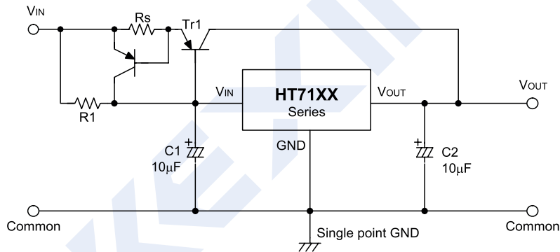
Short-Circuit protection by Tr1
