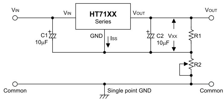
Circuit for increasing output voltage
