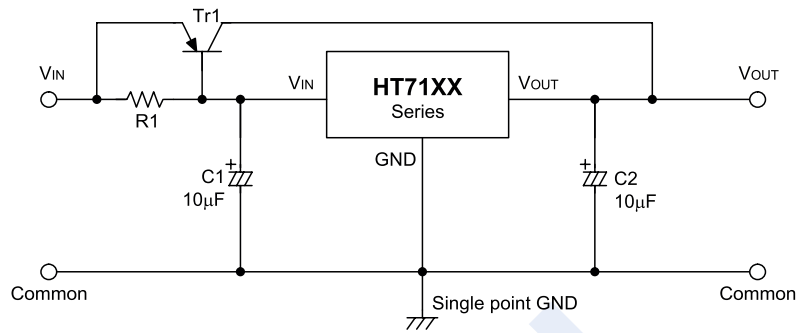
High output current positive voltage regulator
