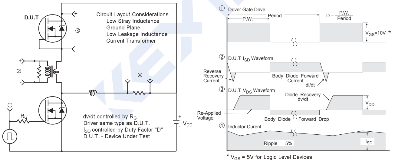
Fig 12. For N-Channel HEXFETS
