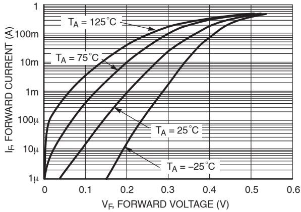
Figure 1. Forward Characteristics
