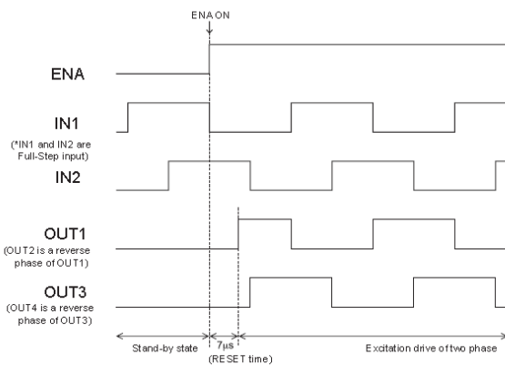
Figure 4 Control Timing
