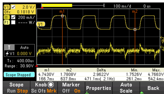
Figure 10. Scope View.
