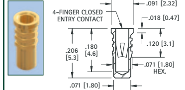
.032 (.56) - .046 (1.17) PIN - PRESS-FIT
