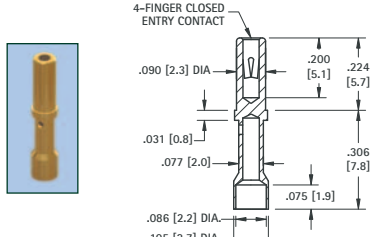
.032 (.81) - .046 (1.17) PIN - CRIMP BARREL JACK
