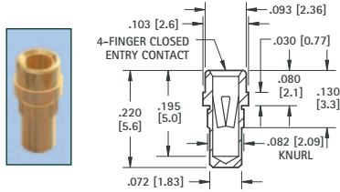
.032 (.81) - .046 (1.17) PIN - PRESS-FIT
