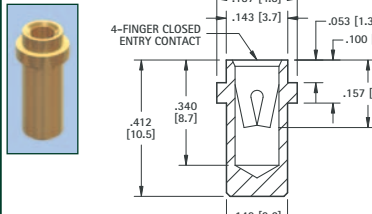
.065 (1.65) - .082 (2.08) PIN - SOLDER MOUNT
