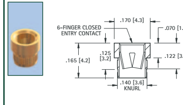
.084 (2.13) - .102 (2.6) PIN - PRESS-FIT
