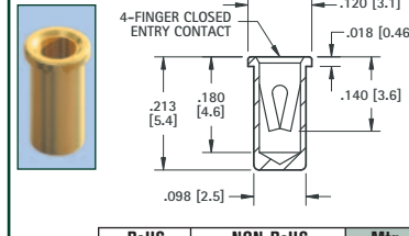
.048 (1.22) - .064 (1.63) PIN - SOLDER MOUNT
