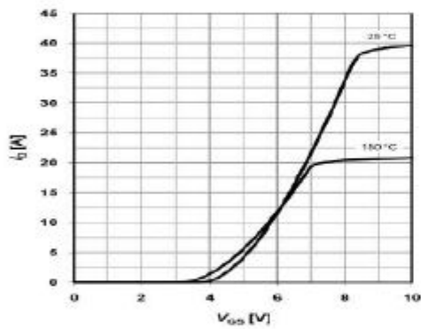
Figure 9. Transfer Characteristics
