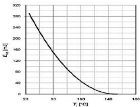
Figure 11. Avalanche Energy Characteristics
