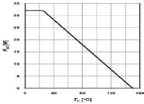
Figure 1. Power Dissipation
