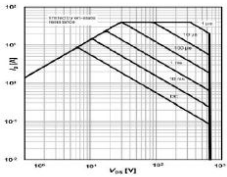
Figure 3. Maximum Safe Operating Area
