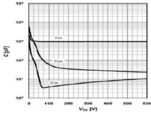
Figure 13. Capacitance Characteristics
