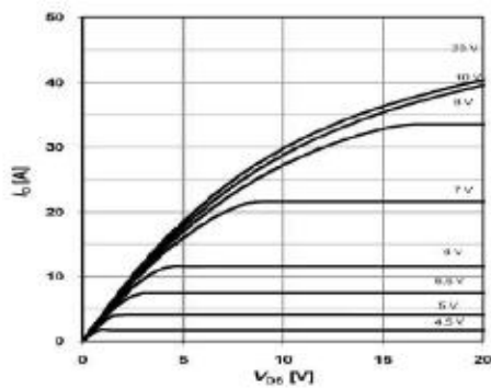
Figure 5. Output Characteristics@25°C
